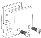
Item no.: LBS-EGC-610 Material: Zinc-alloy Application: Channel Support Thickness: 5-8mm
