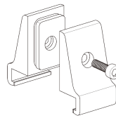
Item no.: OMA05 Material: Zinc-alloy Application: Upmount Clamp Thickness: 6mm
