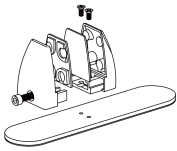
Item no.: HMA82 Material: Zinc-alloy Application: Free Standing Thickness: 5-22mm
