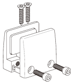
Item no.: OMA01 Material: Zinc-alloy Application: Upmount Clamp Thickness: 5-22mm
