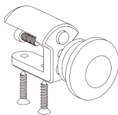
Item no.: OMA02 Material: Zinc-alloy Application: Side Mount Clamp Thickness: 5-22mm
