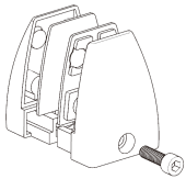
Item no.: SM-RC-618KIT Material: Zinc-alloy Application: Panel Divider Thickness: 5-22mm
